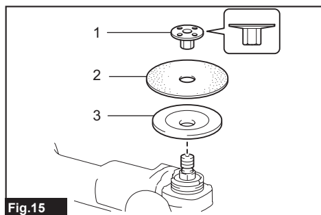
Fig.15 ▶ 1. Sanding lock nut 2. Abrasive disc 3. Rubber pad
